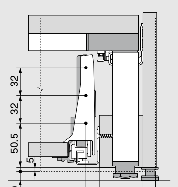
Front dimensions for screw-on assembly
