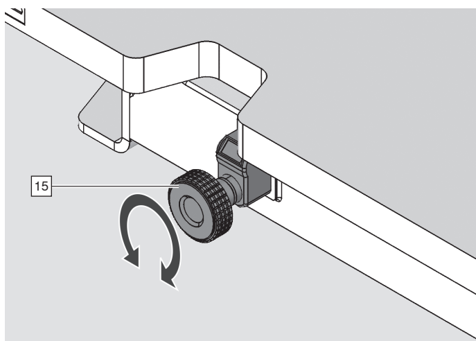
Drilling depth adjustment knob [15] for horizontal drilling. Drilling depth adjustment range: 0 - 50 mm.
