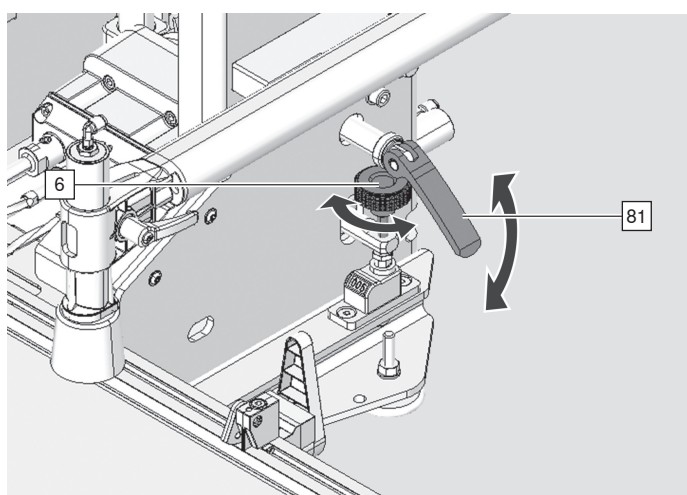
Height adjustment knob [6] for horizontal drilling. Drilling height adjustment range: 6 - 20 mm. A clamping lever [81] secures the setting.
