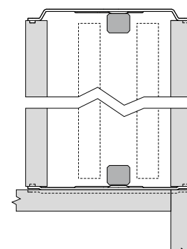
Countertop application
