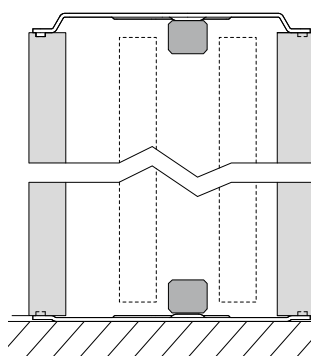
Without toe-kick
