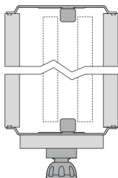
With toe-kick (leg levelers)
