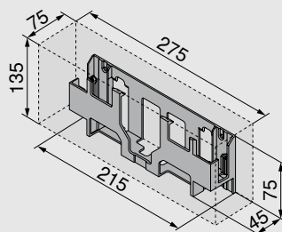
Back panel/wall fixing
