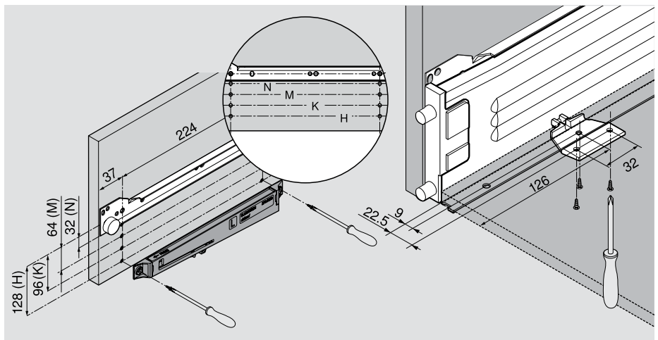
System 32: BLUMOTION unit assembly uses a 32 mm drilling system.
